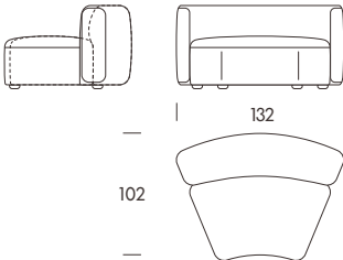
Extension DO15 132×102×65cm
