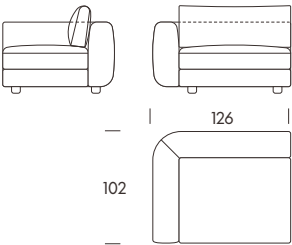
End Unit TR11 126×102×79cm
