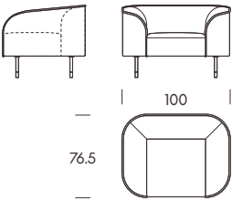
Armchair LM10 100×76.5×67cm
