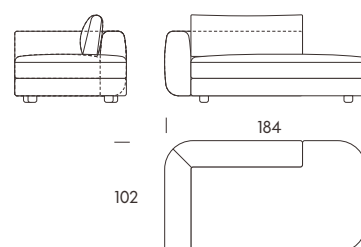
One Seater TR44 184×102×79cm
