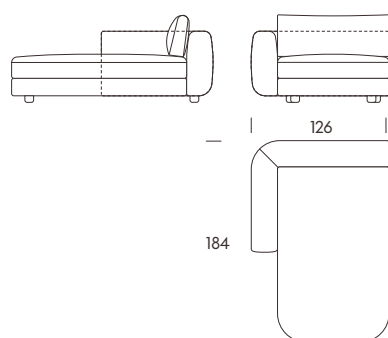
Chaise Longue TR42 126×184×79cm
